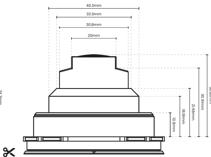
12mm T2.9 Zero-D FF ML Cine
